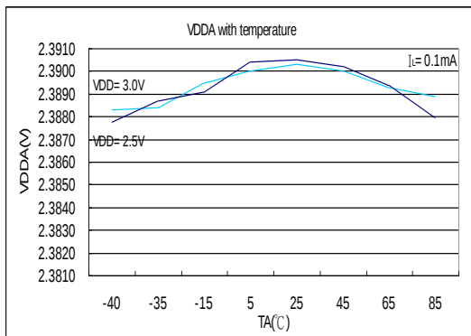
Figure 6.6-3 VDDA I_L=0.1\text{mA} vs. VDD
